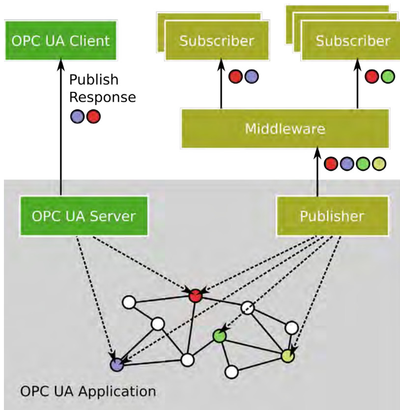
Client/Server and Publish/Subscribe models.
